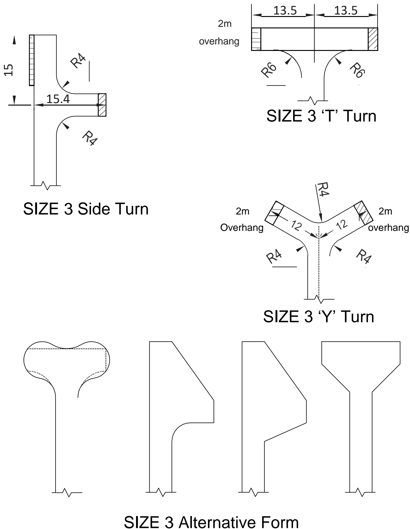
Figure 2 – Residential Adoptable Roads (5.5m wide) - Turning Spaces (All dimensions in metres)
